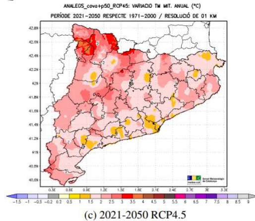
(c) 2021-2050 RCP4.5
