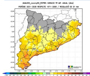
(b) 2021-2030 RCP8.5
