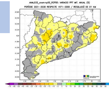
(b) 2021-2030 RCP8.5
