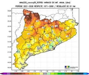
(b) 2021-2030 RCP8.5
