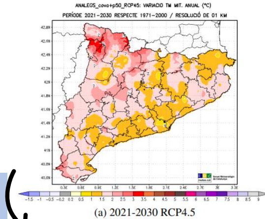
(a) 2021-2030 RCP4.5
