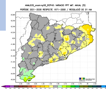
(a) 2021-2030 RCP4.5
