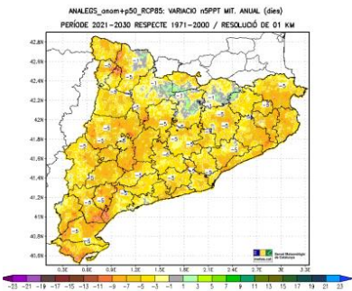
(b) 2021-2030 RCP8.5
