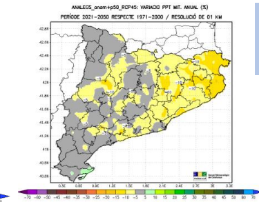
(c) 2021-2050 RCP4.5
