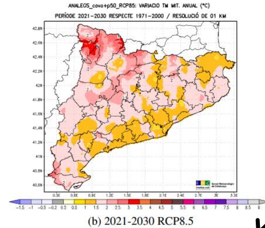
(b) 2021-2030 RCP8.5
