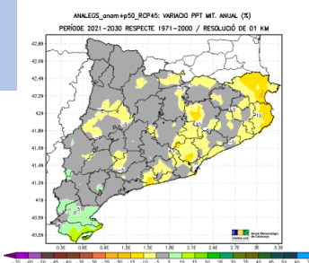
(a) 2021-2030 RCP4.5
