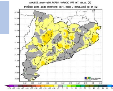
(b) 2021-2030 RCP8.5
