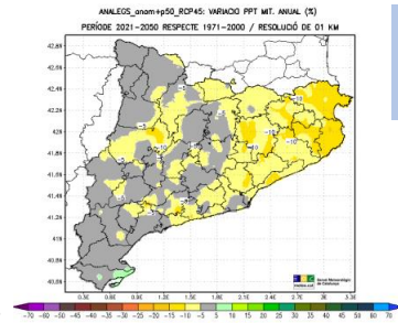
(c) 2021-2050 RCP4.5
